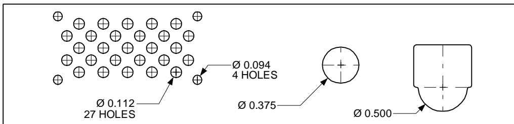
REAR PANEL CUTOUTS
