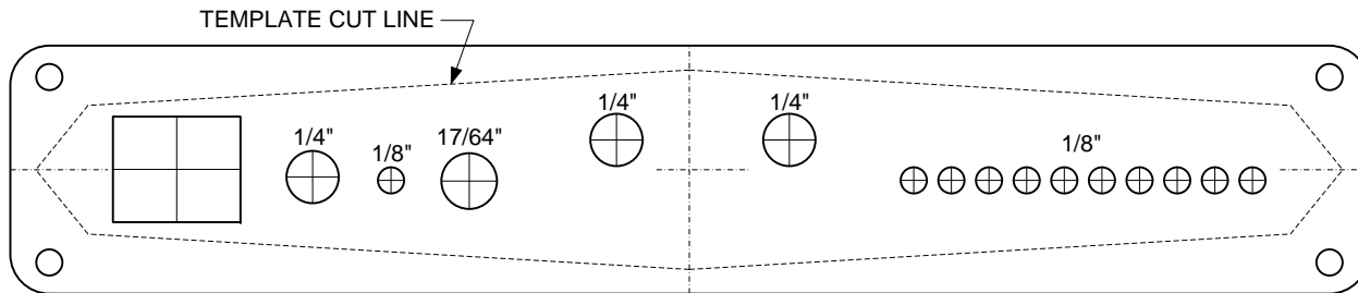
FRONT PANEL
