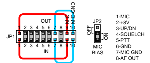
Jumpers: Icom IC-756
