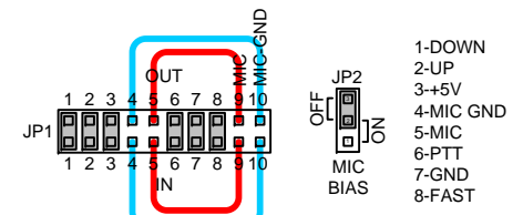
Jumpers: Yaesu FT-857
