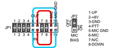
Jumpers: Kenwood TS-480SAT
