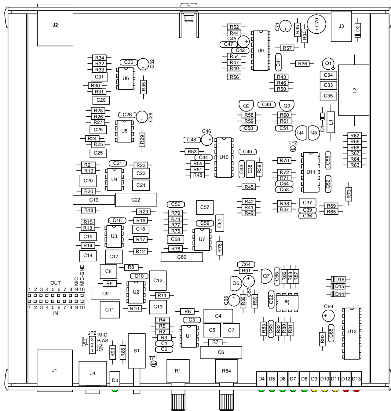
TOP VIEW (TOP PANEL REMOVED)
